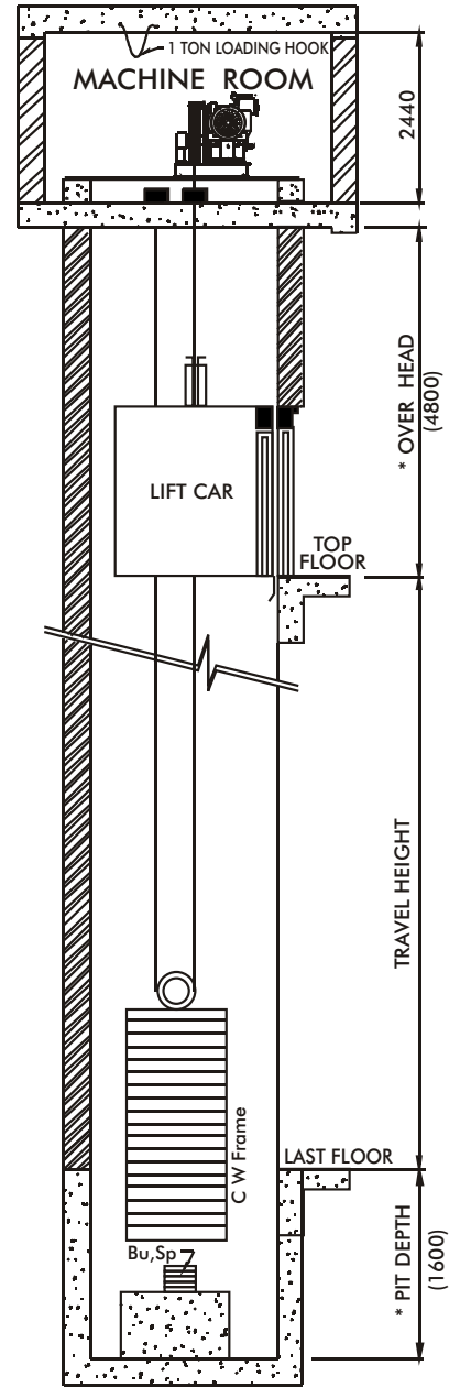
(SECTION : X-X) LIFT WELL
