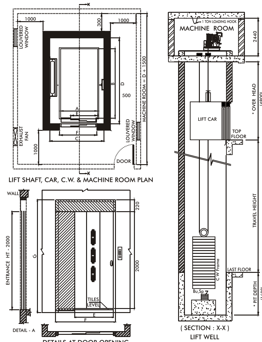
Hospital Lift with Imperforated / Swing / Collapsible Manual Door Std. Speed - 0.35 m/s
