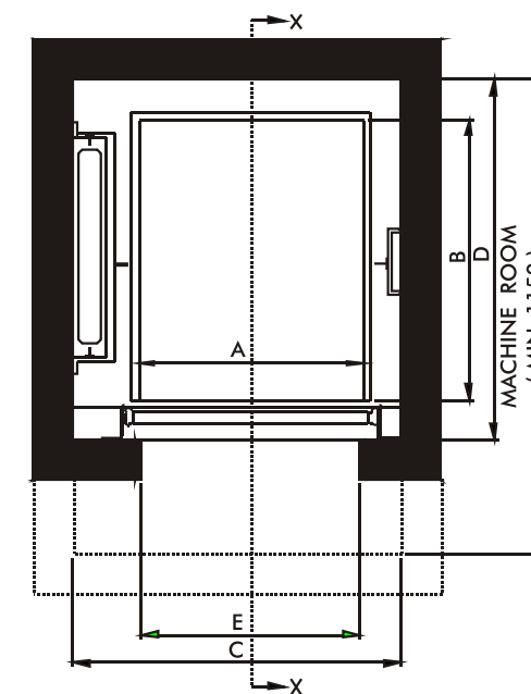
LIFT SHAFT, CAR, C.W. & MACHINE ROOM PLAN
