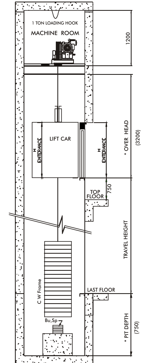
( SECTION : X-X ) LIFT WELL
